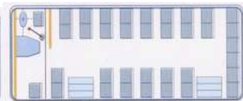
4200mmWB - 35 seats 2 doors (2 x 2 layout)
